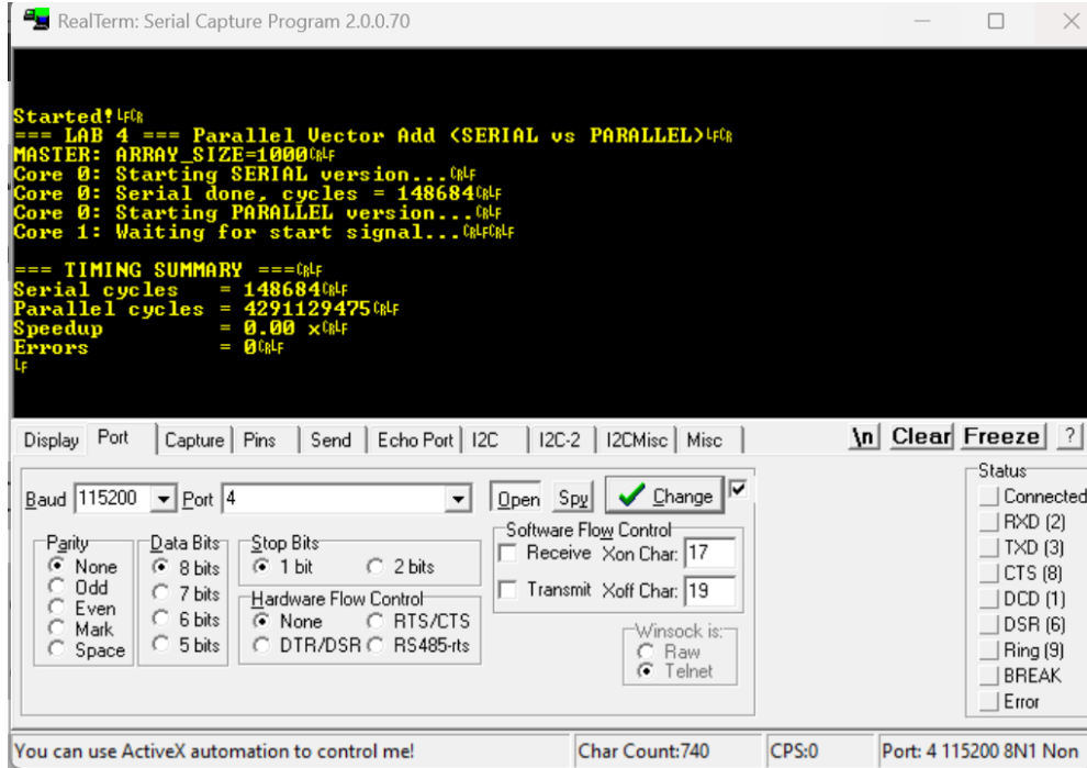
Figure 8: UART output for the parallel vector addition with ARRAY_SIZE = 1000 .
