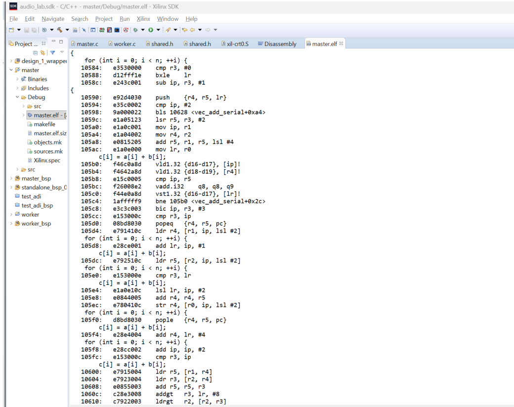
Figure 10: Disassembly of the serial baseline showing ARM NEON SIMD instructions ( vld1.32 , vadd.i32 , vst1.32 ).
