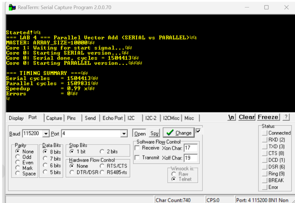
Figure 9: UART output for the parallel vector addition with ARRAY_SIZE = 10000 .
