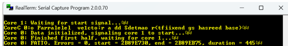
Figure 11: UART output showing correct parallel execution on both cores (Master and Worker).
